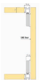
Door Flush Version Thickness of door: 16-32mm
