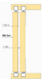
Concealed Version Thickness of door: 16-32mm
