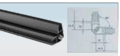
OPS-M3 10mm BM ₹ 1,192 90° Magnetic Seal
