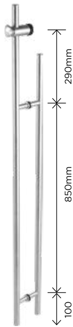
OGHL-55-25x1340 SSS Glass Door Handle with locking function
