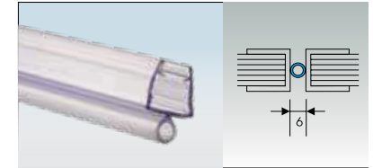
OPS-5 STD ₹ 270 Soft Nose Seal
