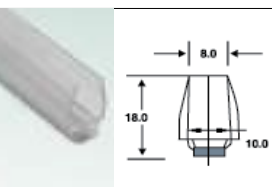
OPS-SL-BR-11 12mm STD ₹ 832 Brush Seal (Central)
