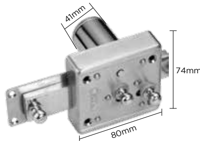
OZ-NL-55 STD SSS ₹ 1,199 Interlock with 3 Stroke
