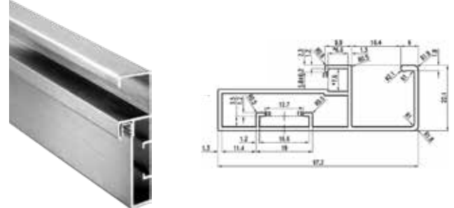
Aluminium Handle Frame Profile
