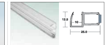
OZOM-SL-BR-22N-10ft 12m STD ₹ 832 Brush Seal (Sliding Doors)
