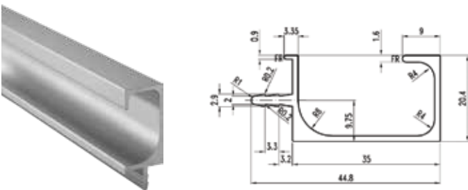
Aluminium Handle Frame Profile
