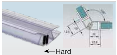
OPS-M2 8mm STD ₹ 972 135° Magnetic Seal
