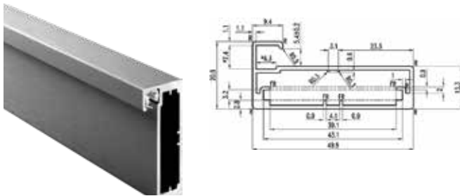
Aluminium Frame Profile
