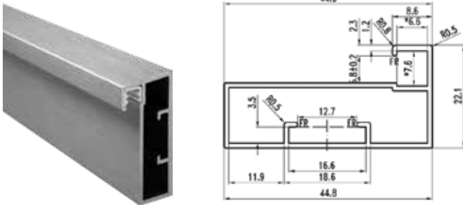
Aluminium Frame Profile
