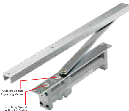
CDC-3800 STD SILVER ₹ 5,610 CONCEALED DOOR CLOSER
