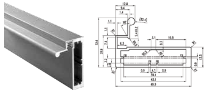
Aluminium Handle Frame Profile
