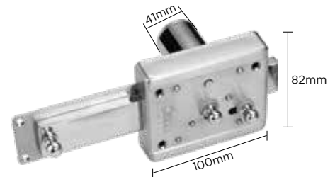
OZ-NL-66 STD SSS ₹ 1,419 Interlock with 6 Stroke
